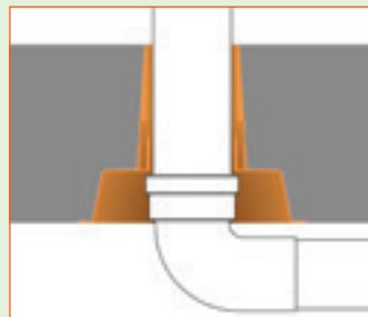
Cross-section of QuelCast Cast In Fire Collar installed with a Manifold on the Bottom
