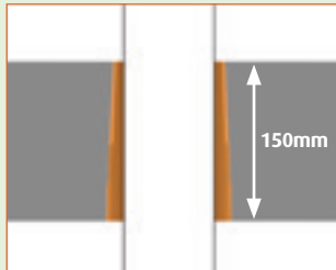
Cross-section of QuelCast Cast In Fire Collar cut to suit a 150mm floor slab
